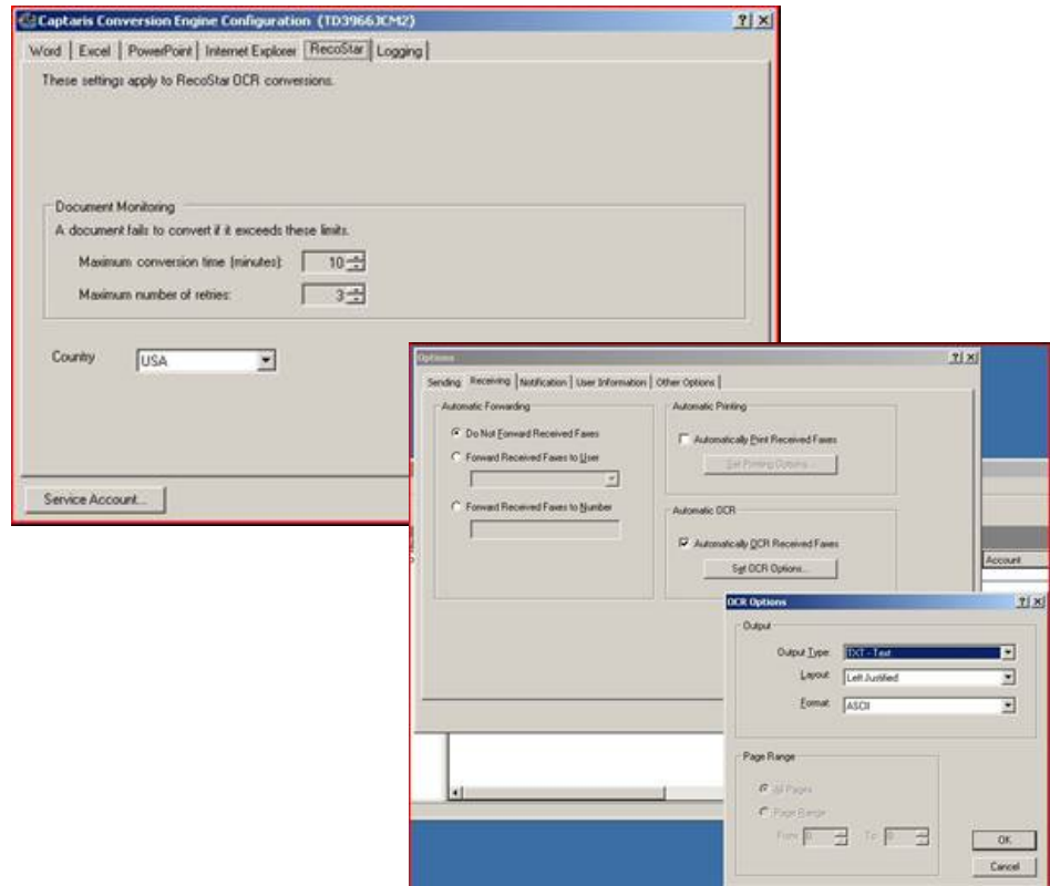
Figure 10: New RecoStar OCR engine
